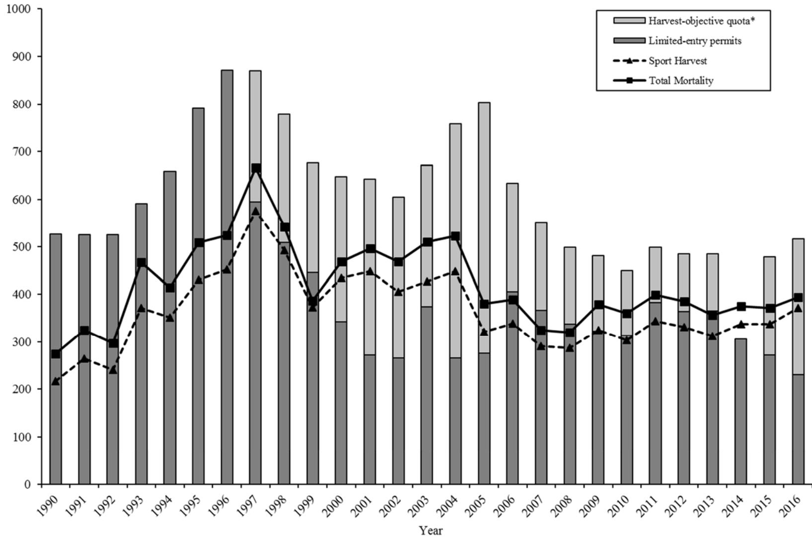
Statewide cougar mortality and harvest objectives, 1990 through 2016.
