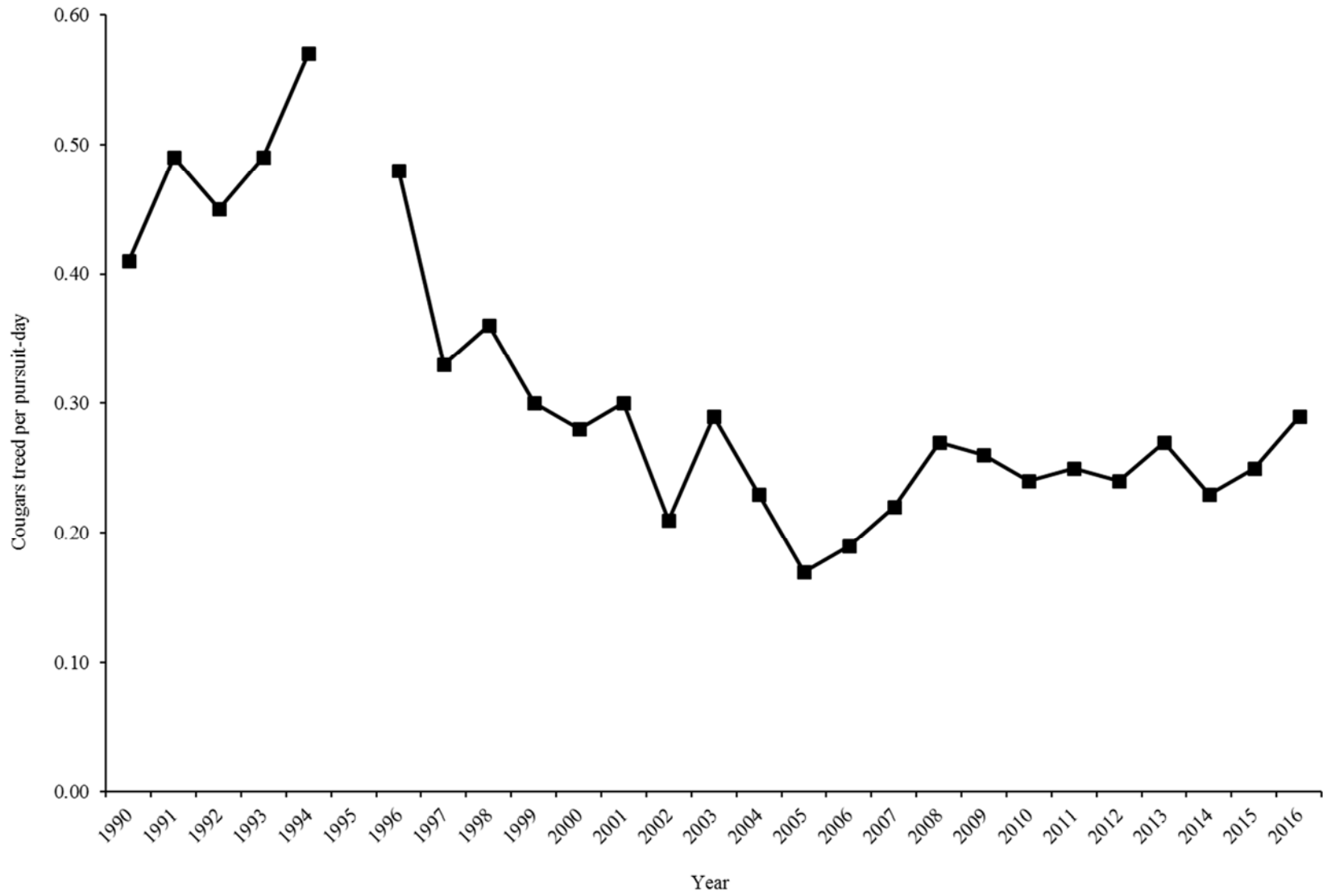
Statewide cougars treed per pursuit-day, 1990 through 2016.
