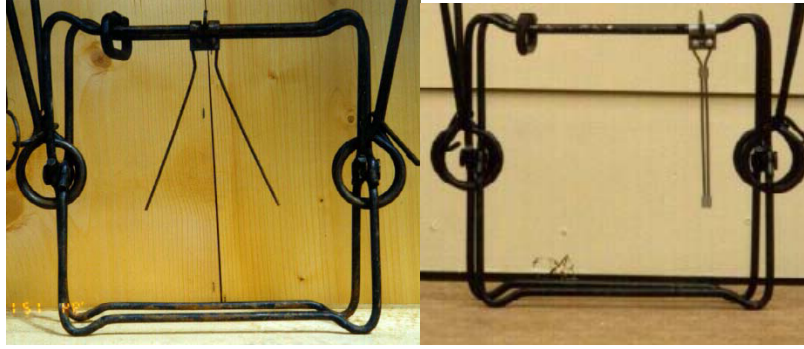
Figure 2. Standard V-trigger conibear trap and modified conibear trap.
